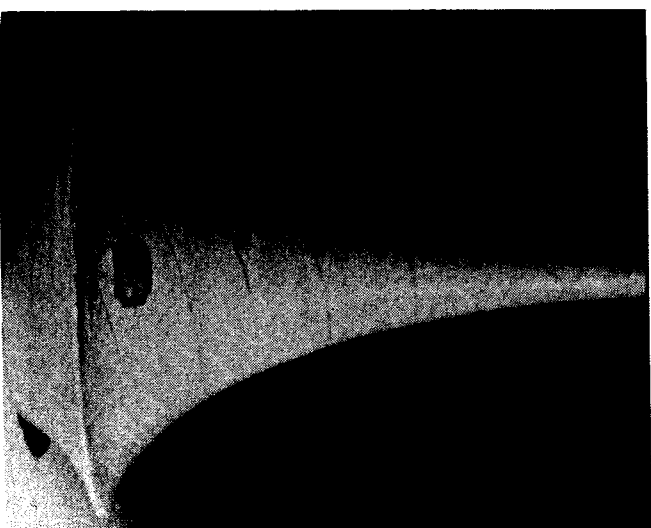
(b) the parabolic pseudospherical surface or "pseudoshell";
