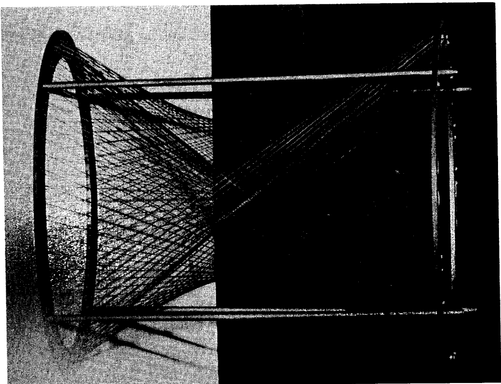
FIGURE 5. Hyperboloids are the simplest expression of multiply-connected, self-similar spiral action. Shown is one of the pedagogical models used in the teaching of the LaRouche-Riemann method in physical geometry .
