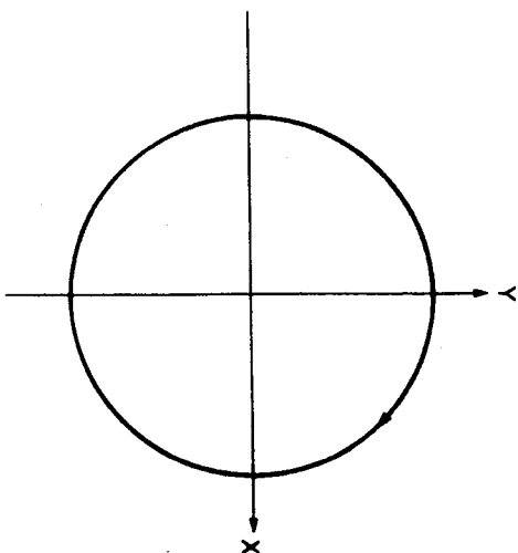
FIGURE 1. Circular Action The smallest possible circumference (minimum) encloses the greatest possible area (maximum). This "isoperimetric principle" is derived from the Maximum-Minimum principle. It is a question here of the characteristics of the action , and not of the circle as such, which is only an image of the action.
