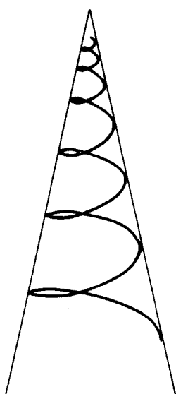
FIGURE 3. Self-similar spirally formed action connects the circular action in time with growth.
