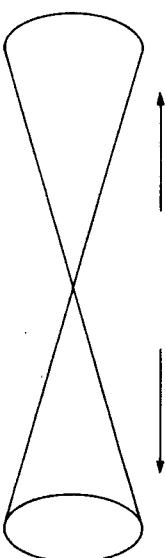
FIGURE 4. The double cone, as it is defined by self-similar spiral action in opposite directions.
