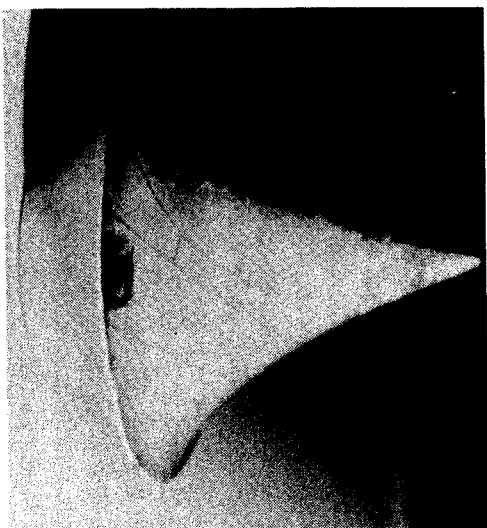
(a) the elliptical-pseudospherical surface of rotation, which corresponds also to the surface of rotation of the caustic;
